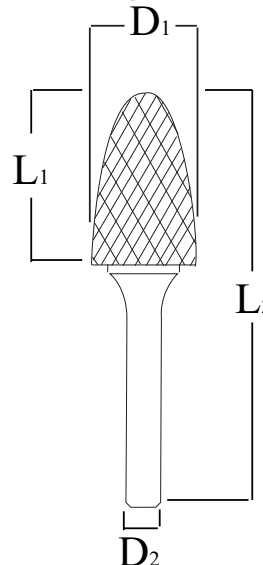
Bur Diagram
